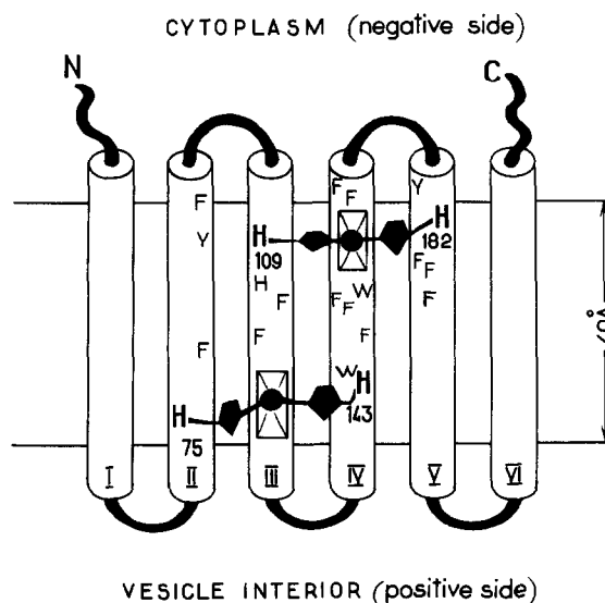
Fig. 2. Model for the molecular organization of cyt. b -561 of chromaffin granules. The proposed histidine ligands of the heme irons and aromatic residues close to the hemes are indicated using the single-letter code. The approximate dimensions of the hemes and the membrane are respected in the model.
